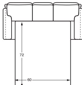
628-015 Queen Sleeper* 628-0152 2-Over-2 Queen Sleeper* 86W 40 D 38 H 26 AH 21 SH
