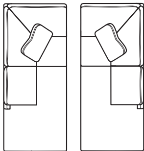
628-0B3 LSF Bumper Section 628-0B4 RSF Bumper Section 40W 94 D 38 H 21 SH
